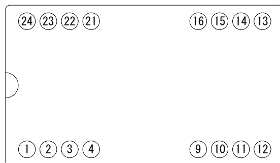
<Pin Location (Top View) >
